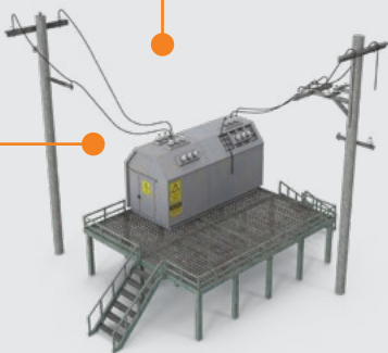
HV poles, MV Poles, Pad-Mounted Transformer
